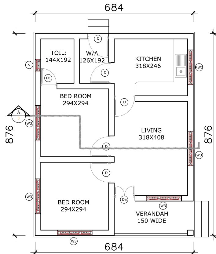
1 GROUND FLOOR PLAN
