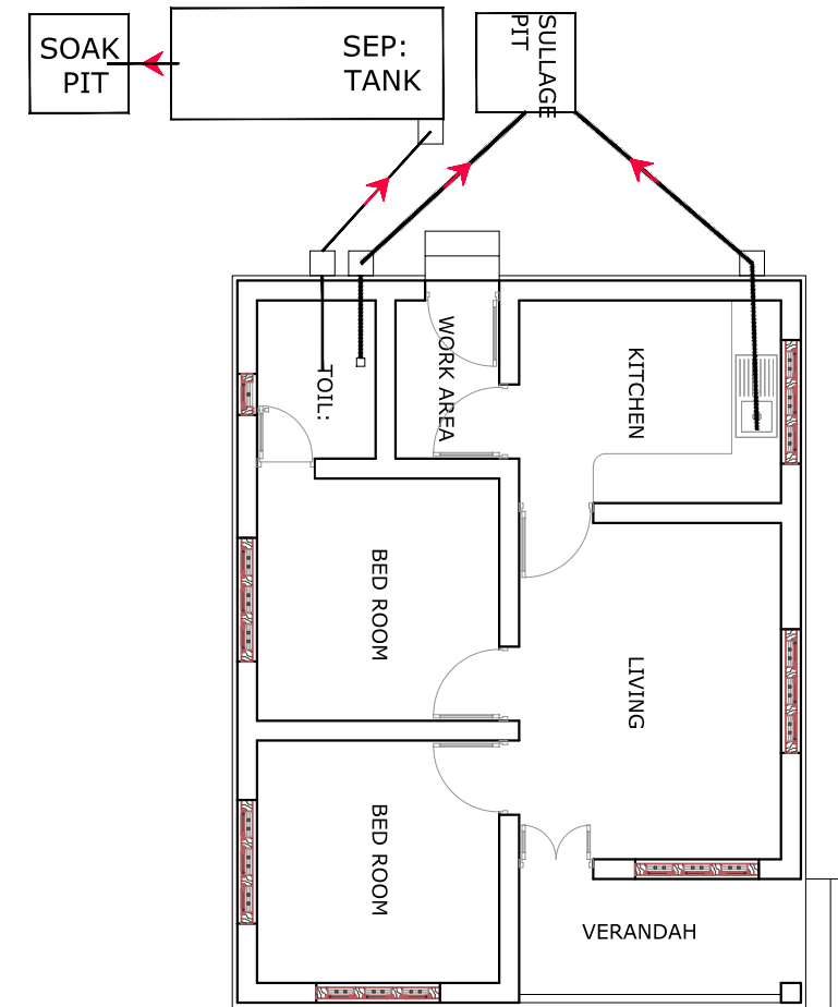
5 GROUND FLOOR SERVICE PLAN
