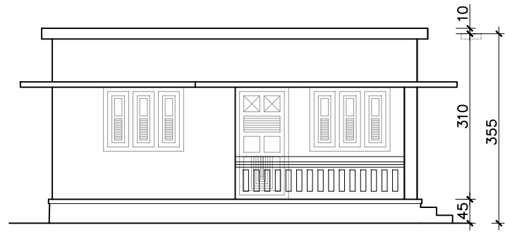
2 FRONT ELEVATION
